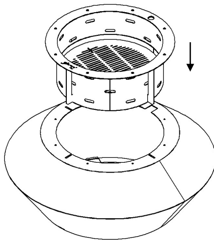
Figure 2 – Place the combustion zone
